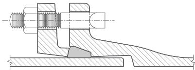
Mechanical Joint (3"-24")
