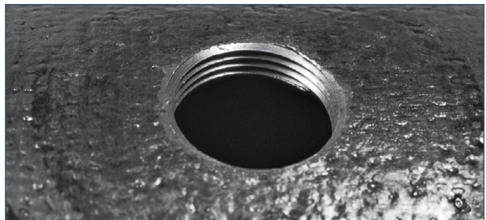
Forces exerted during pull-out tests, when sufficient, resulted in failure of the corporation stop, not the Ductile Iron Pipe or threads. The top photo shows leakage at the plug key of the corporation stop. Ultimate failure occurred to the corporation stop’s threaded connection for the service line. The undamaged Ductile Iron Pipe and threads are shown in the photo below.
