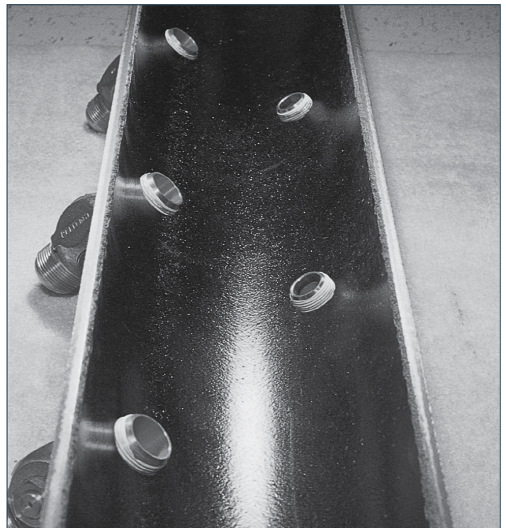
This cutaway view of the inside of a tapped Ductile Iron Pipe clearly shows that the corporation stops do not damage the cement-mortar lining of the pipe.
