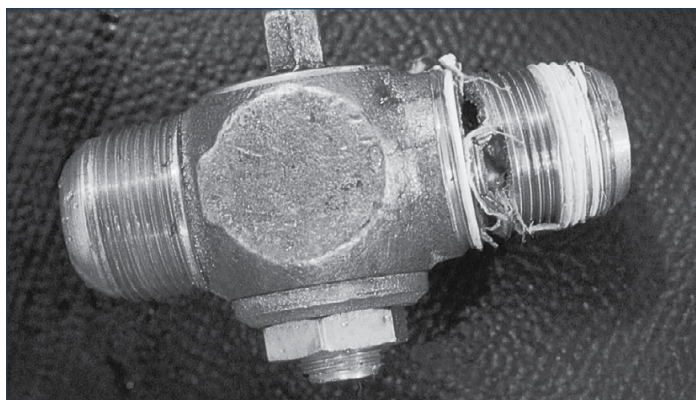
As was the case in the pull-out tests, sufficient cantilever forces damaged the corporation stop, causing the leakage seen in the photo above (top). Damage to the corporation stop is shown above (bottom).
